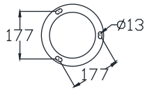
Installation plate
