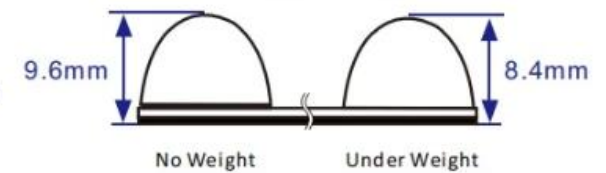
Bumper Height
