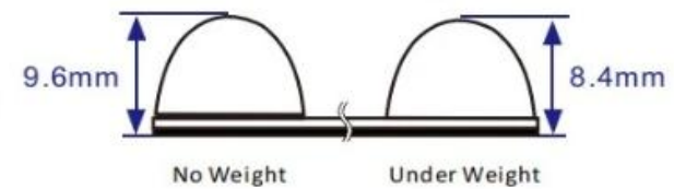
Bumper Height
