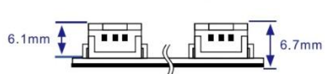
Terminal Height
