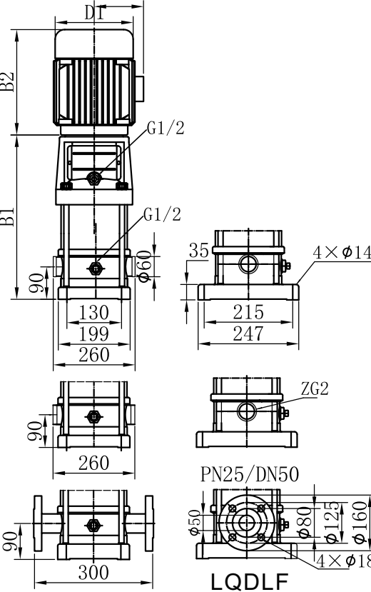
(Installation drawing)
