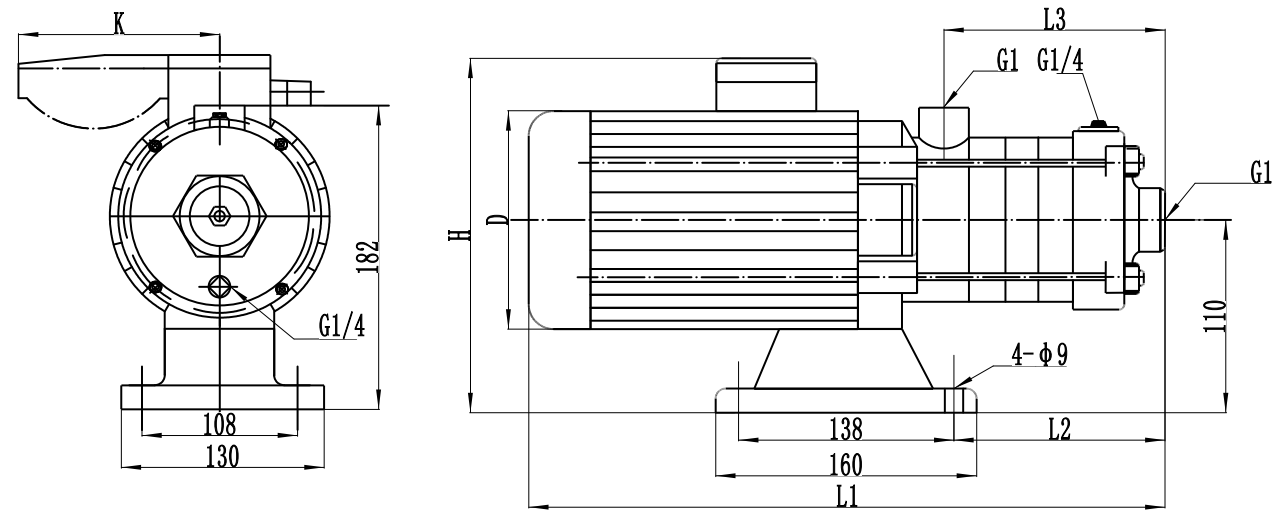
(Installation drawing)
