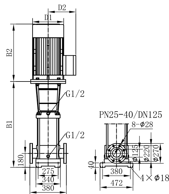
(Installation drawing)
