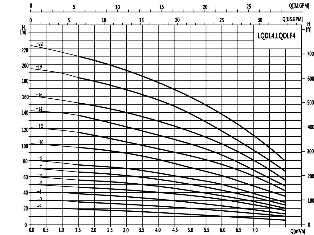
(Performance curve)
