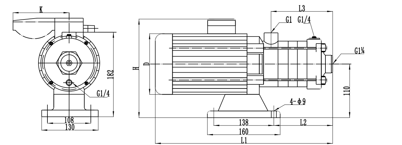
(Installation drawing)
