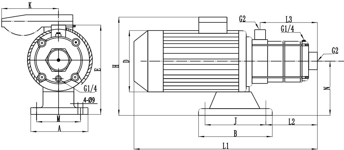
(Installation drawing)
