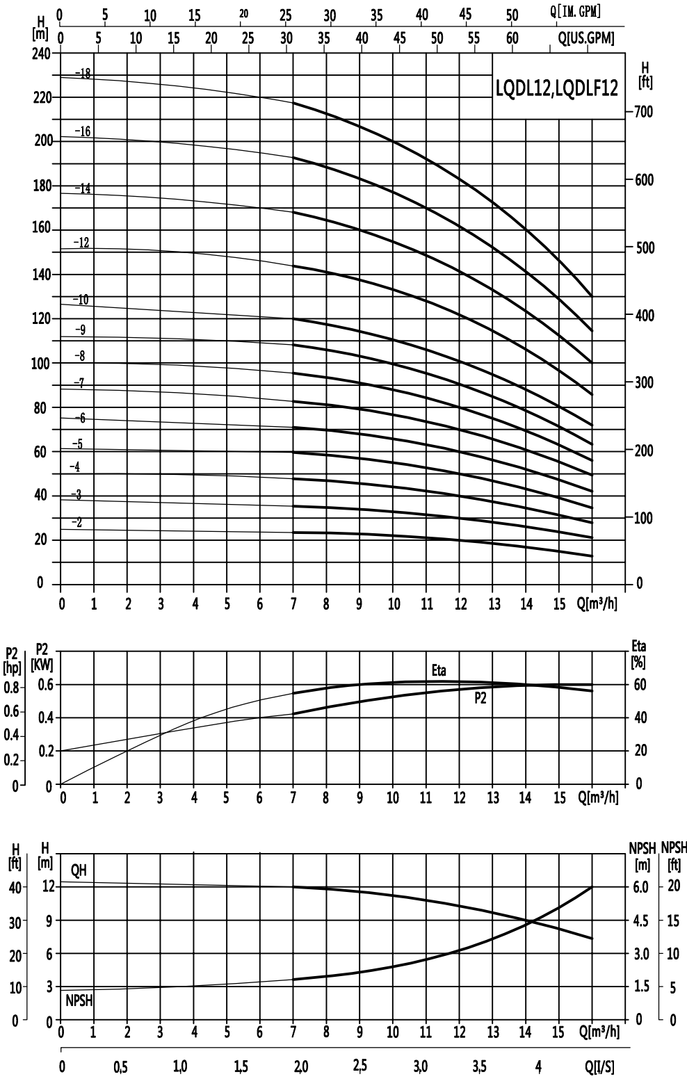
(Performance curve)
