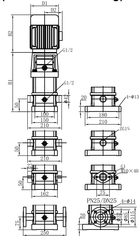
(Installation drawing)
