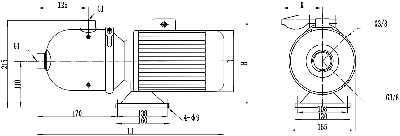
(Installation drawing)
