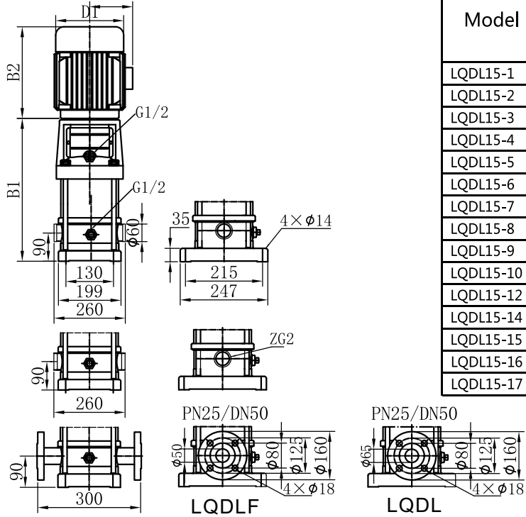
(Installation drawing)
