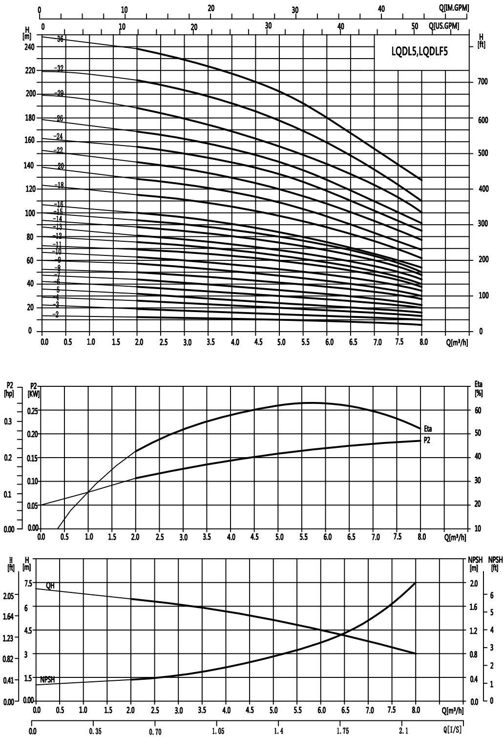
(Performance curve)
