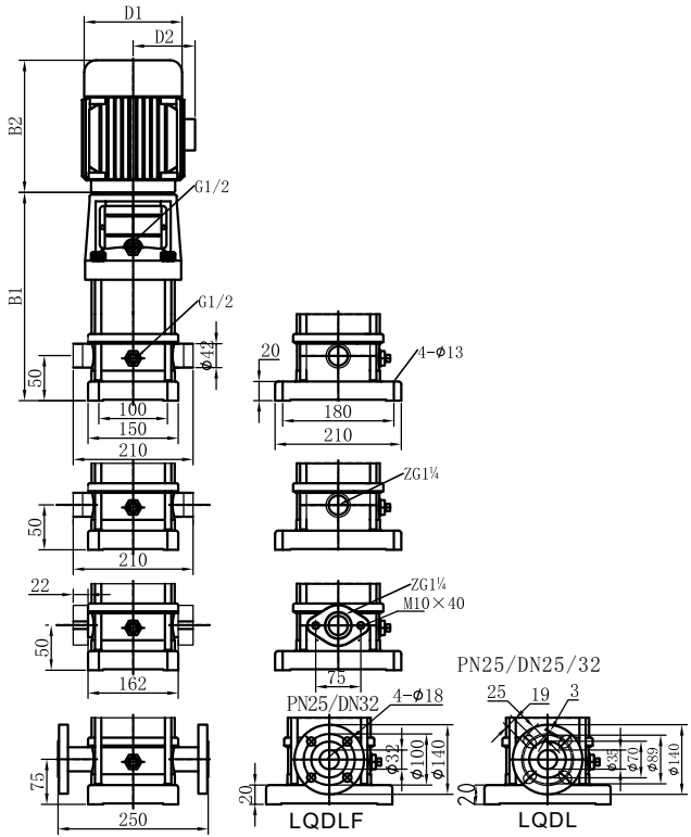
(Installation drawing)
