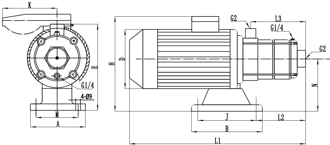
(Installation drawing)
