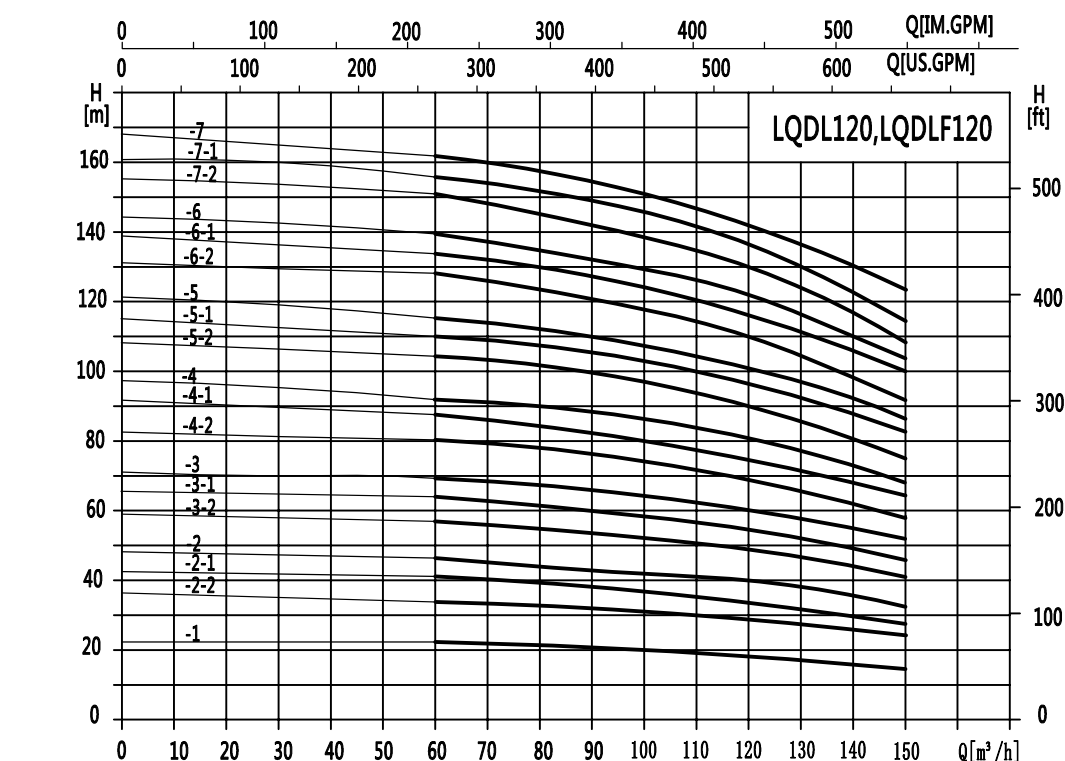
(Performance curve)
