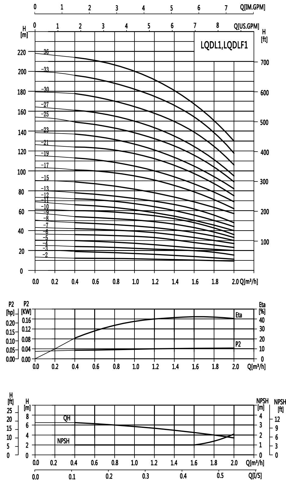
(Performance curve)
