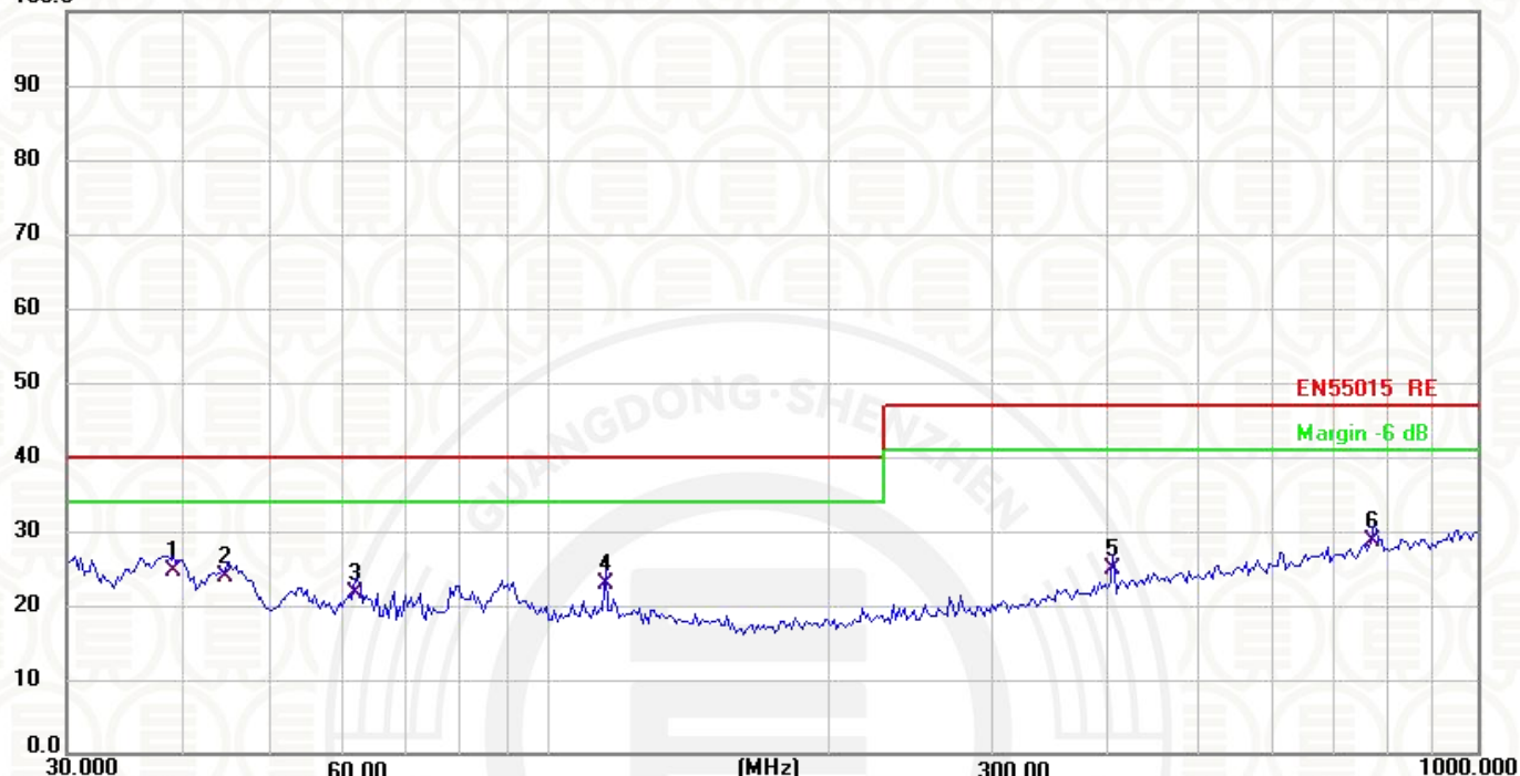
Test Graph 100.0 dBuV/m
