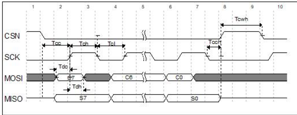
Picture 5-6 SPI Sequence Diagram of Parameters
