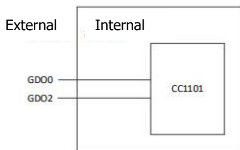
Picture 5-2 GDO0, GDO2 Local Connection Diagram
