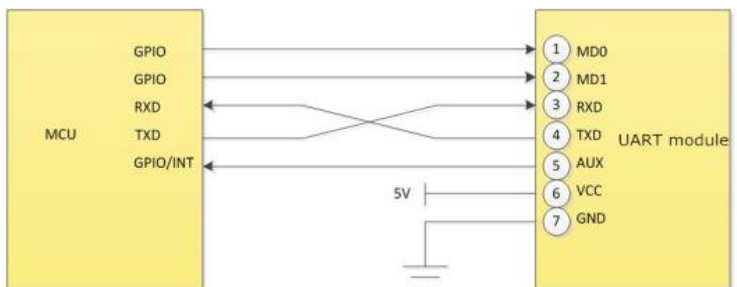
0-1 Recommended Connection Diagram
