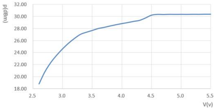
Figure 5-7 Power versus voltage
