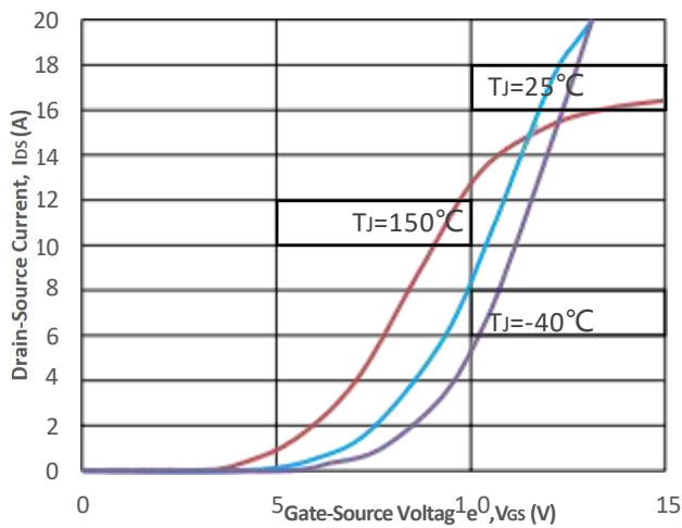
Fig5. Transfer Characteristic
