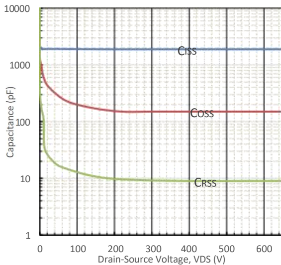
Fig11. Capacitances vs. Drain-Source
