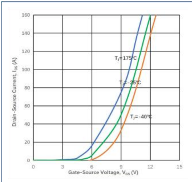
Figure 5 Transfer Characteristic
